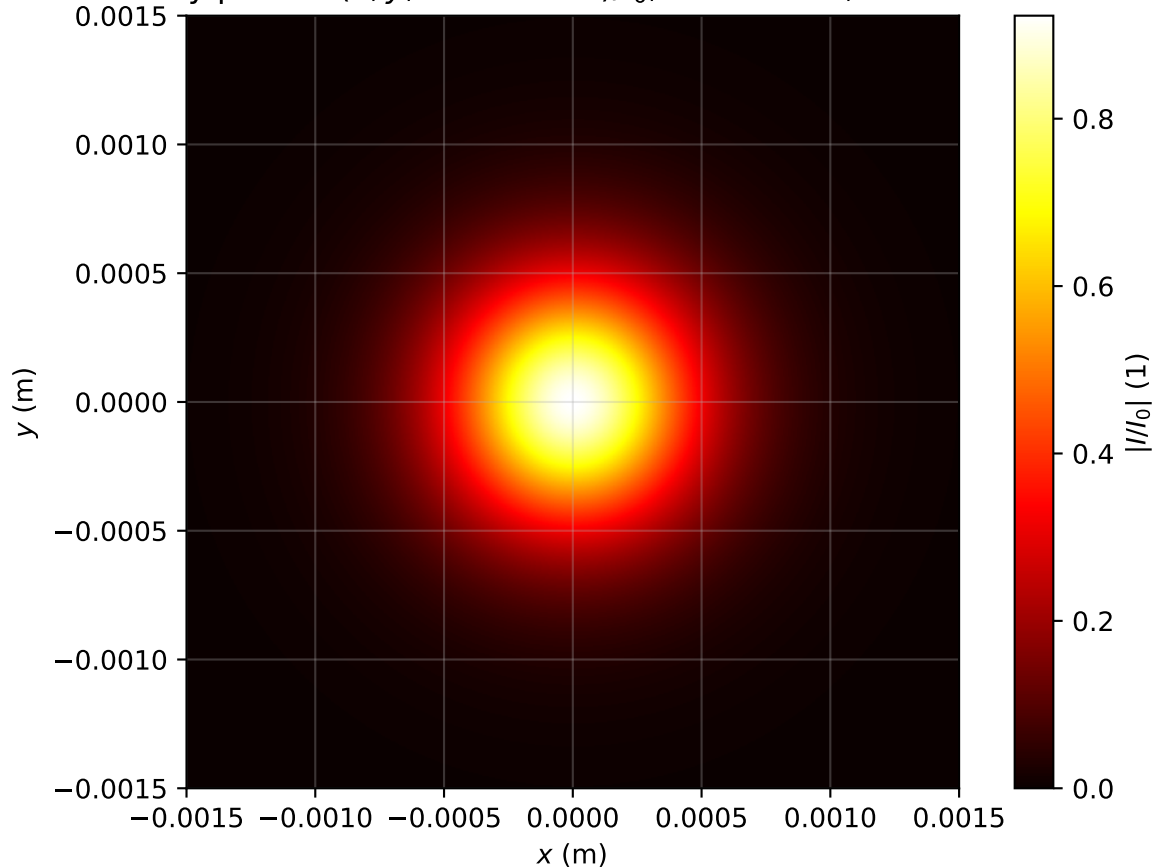
Intensity profile I(x, y, z = 2.070m)/I_0 , P_{in}=0.6P_{cr} , artificial time
